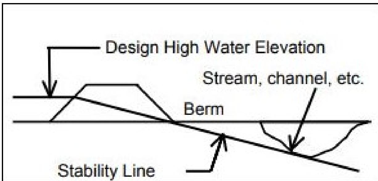
Figure 1. Relative location of dike to stream, channel, ditch, borrow area, slough, swale, gully, etc.
